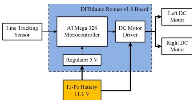
Figure 4. Hardware configuration
