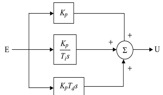
Figure 2. Continuous-time PID controller [6]
