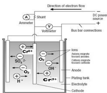
Gambar 1. Prinsip kerja electroplating [2]
