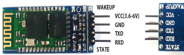
Gambar 3. Modul bluetooth HC-06
