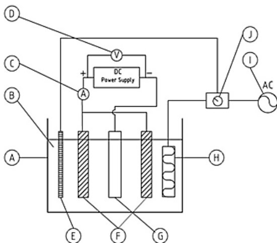
Gambar 2. Instalasi electroplating
