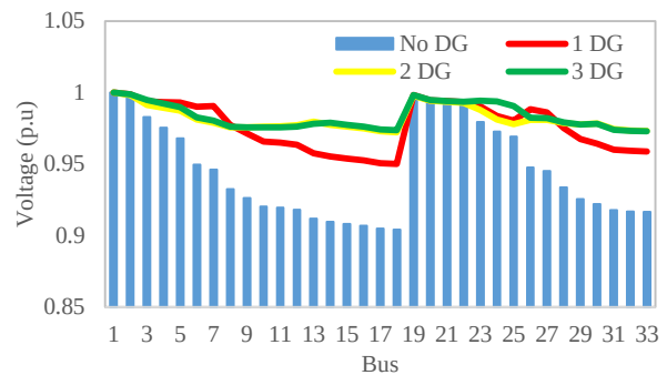
Figure 9. Comparison of the voltage profile of each scenario on IEEE 33-bus test system
