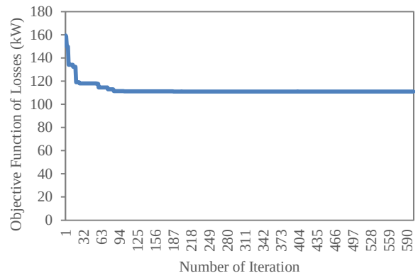
Figure 3. The best convergence graph of placement optimization and wind-based DG capacity to minimize power losses by the FPA method
