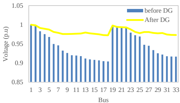
Figure 6. Voltage profile test system IEEE 33 bus
