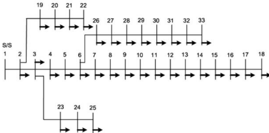
Figure 2. One Line Diagram Test System IEEE 33 bus
