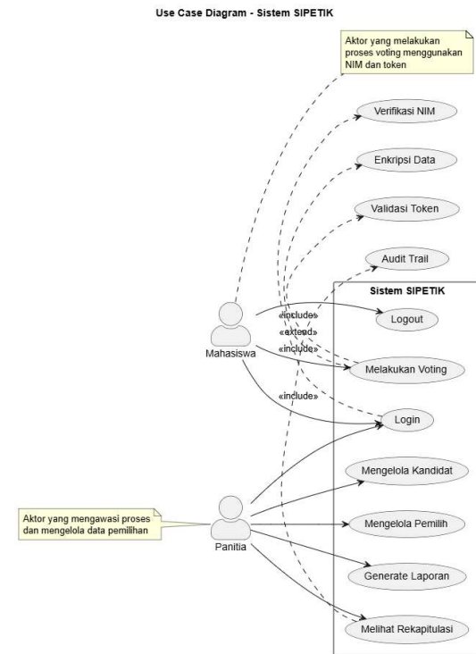
Gambar 2. Use Case Diagram SIPETIK
