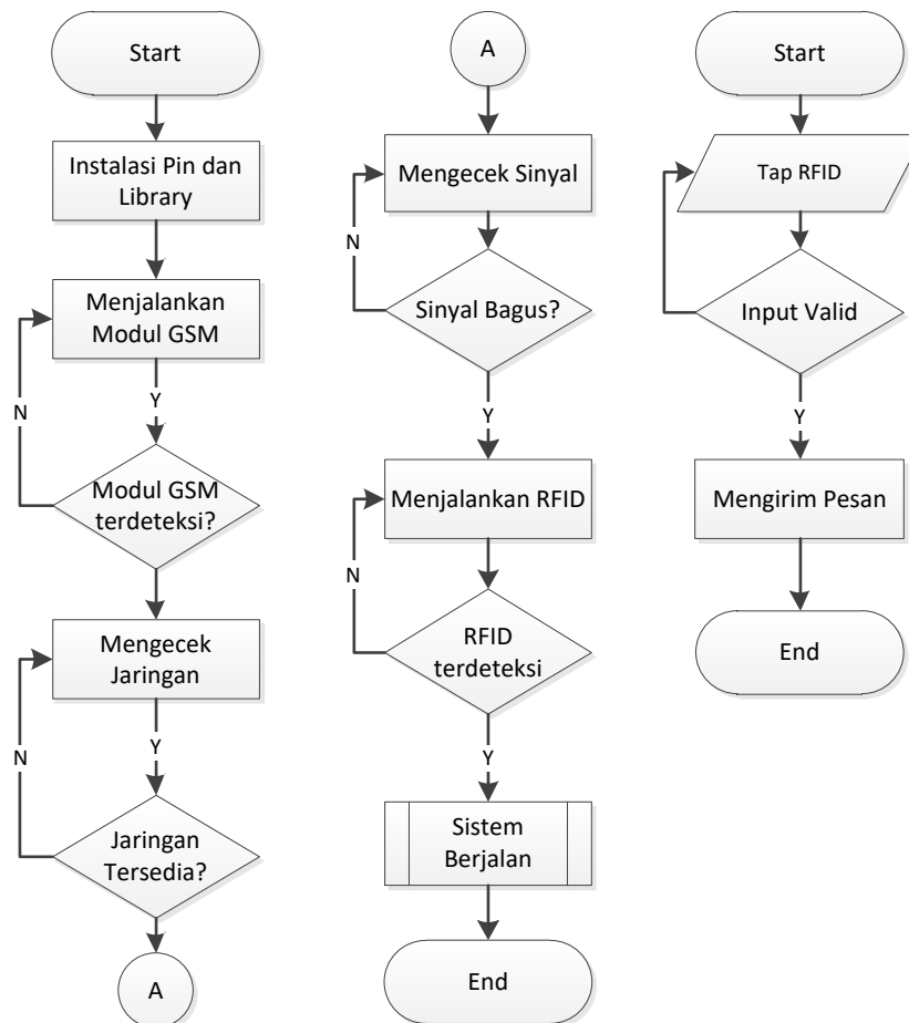
Gambar 3. Flowchart Program Arduino IDE
