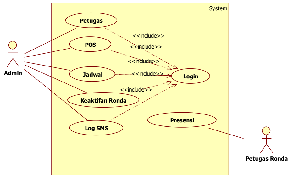
Gambar 4. Use case diagram sistem monitoring
