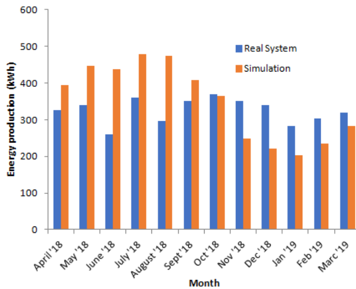
Figure 9. Comparison of energy output between simulation and the real installation system
