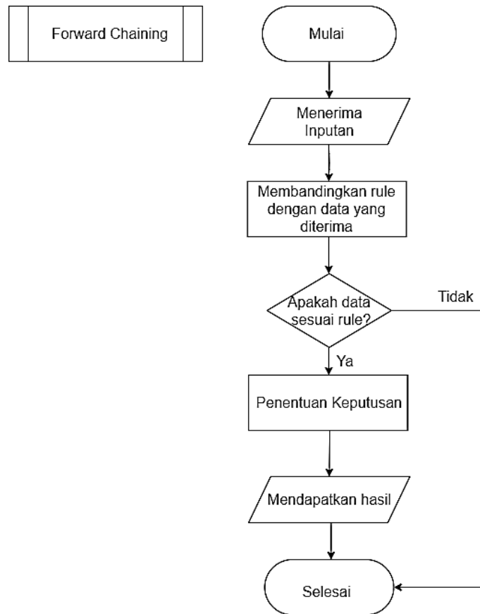
Gambar 4. Flowchart Forward Chaining
