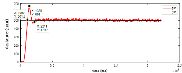
Figure 17. Fuzzy control response for distance 0 – 500 mm.
