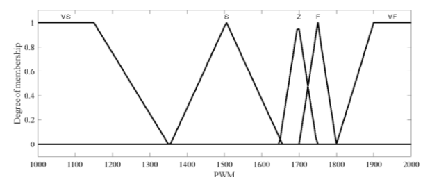
Figure 8. Membership function output PWM
