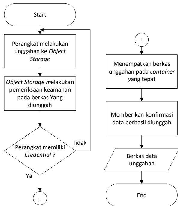
Gambar 3. Diagram alir object storage
